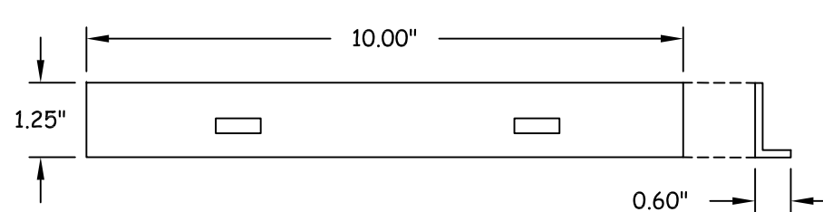
12 BASE ANGLE 1/8" STAINLESS STEEL
