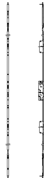
13 3 POINT LOCK SYSTEM STEEL
