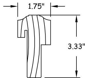
10 WEATHERSTRIP Q-LON
