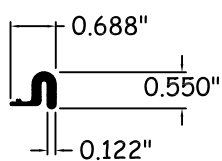
10 WEATHERSTRIP Q-LON
