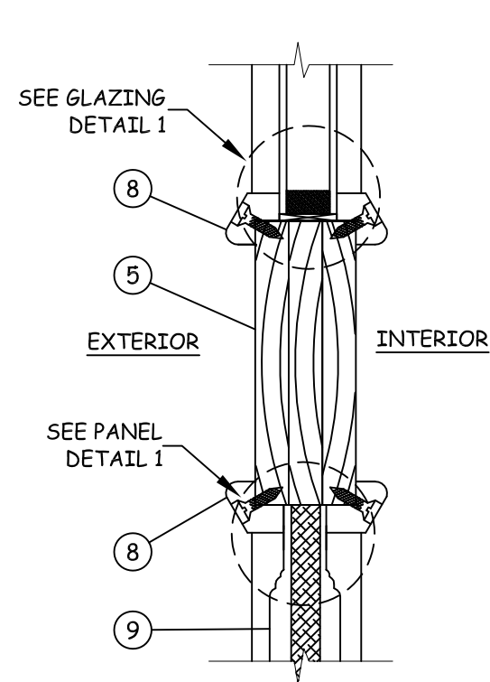
D 4 VERTICAL SECTION MIDRAIL- GLAZED & OPAQUE
