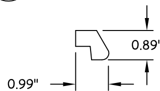
8 GLASS STOP MAHOGANY
