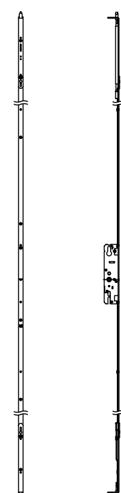
14 2 POINT LOCK SYSTEM STEEL
