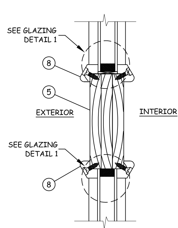
E 4 VERTICAL SECTION MIDRAIL-GLAZED
